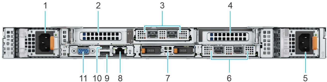
Figure 16. Rear view of the no backplane configuration system *
