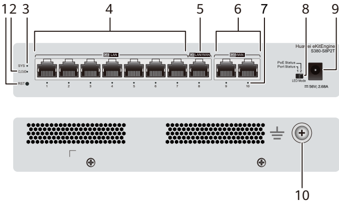
Figure 4-5 S380-S8P2T appearance
